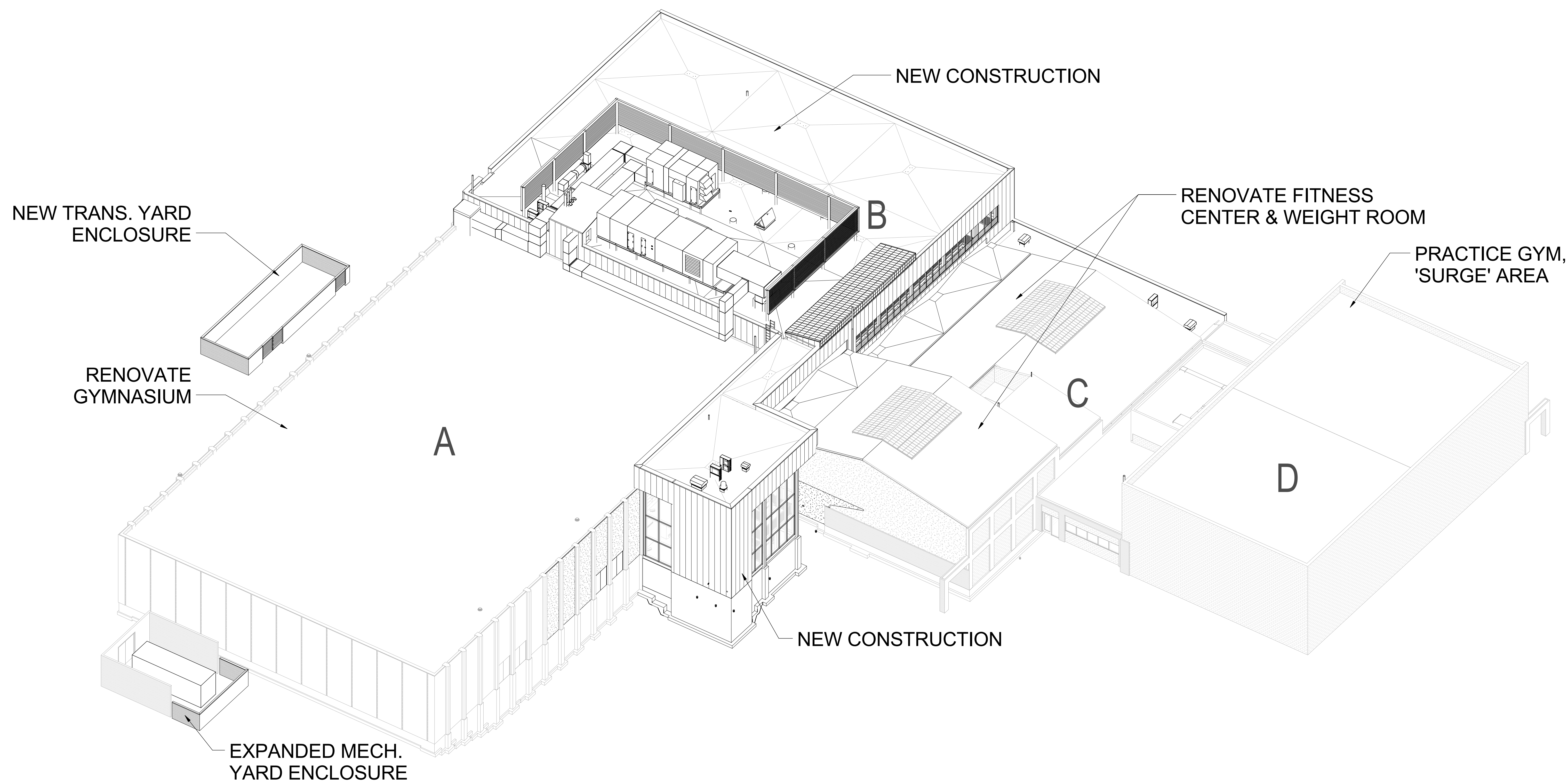
2 FOR REFERENCE ONLY - NEW CONSTRUCTION NORTH WEST SCALE:
