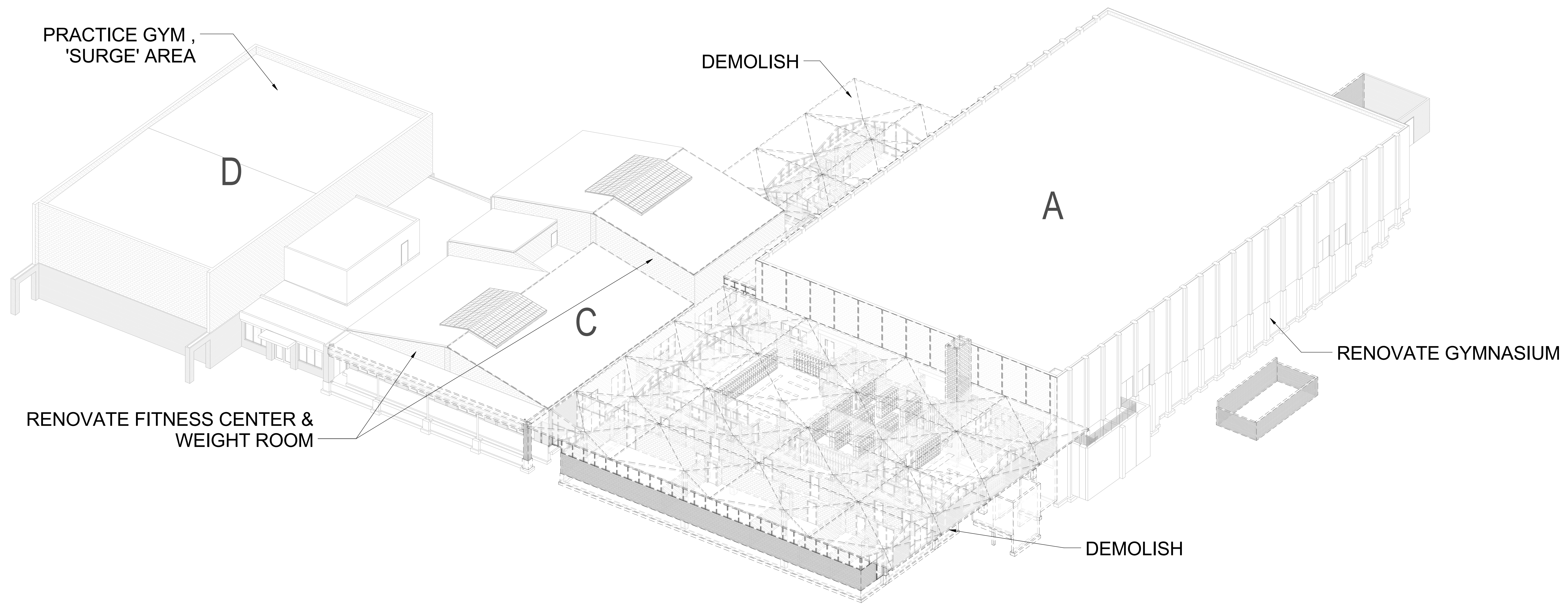
1 FOR REFERENCE ONLY - DEMOLITION SOUTH EAST CORNER SCALE:
